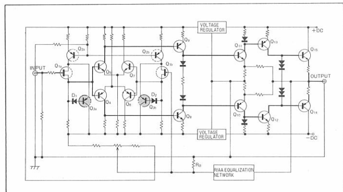
Fig. 1. DIAGRAM OF EQUALIZER AMPLIFIER
