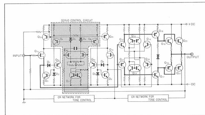
Fig. 2. DIAGRAM OF SERVO CONTROLLED HIGH-LEVEL AMPLIFIER
