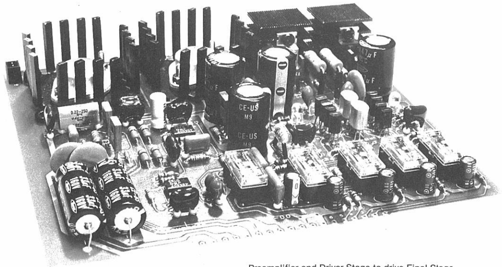
Pre-amplifier and Driver Stage to drive Final Stage. Relays to switch Filter Circuitry is seen in foreground right. MOS FET Driver with Heat Sink is seen in rearward left.
