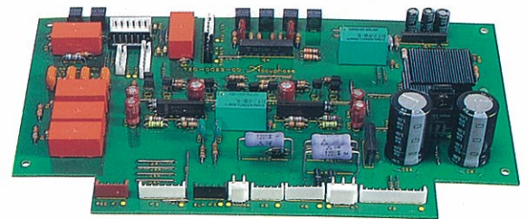
Circuit board incorporating peak power meter driving circuit, protection circuit, and headphone amplifier circuit.
