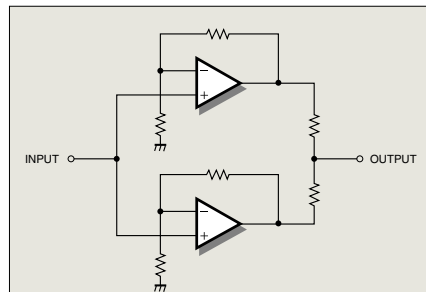
Fig. 2 Circuit diagram of line amplifier (one channel)
