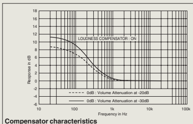
Compensator characteristics
