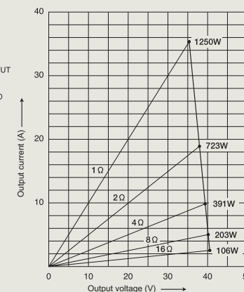
Figure 2 Load impedance vs. output power (output voltage/output current)
