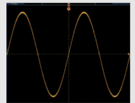
Photo (c) PS-510 output waveform (distortion approx. 0.22%)
